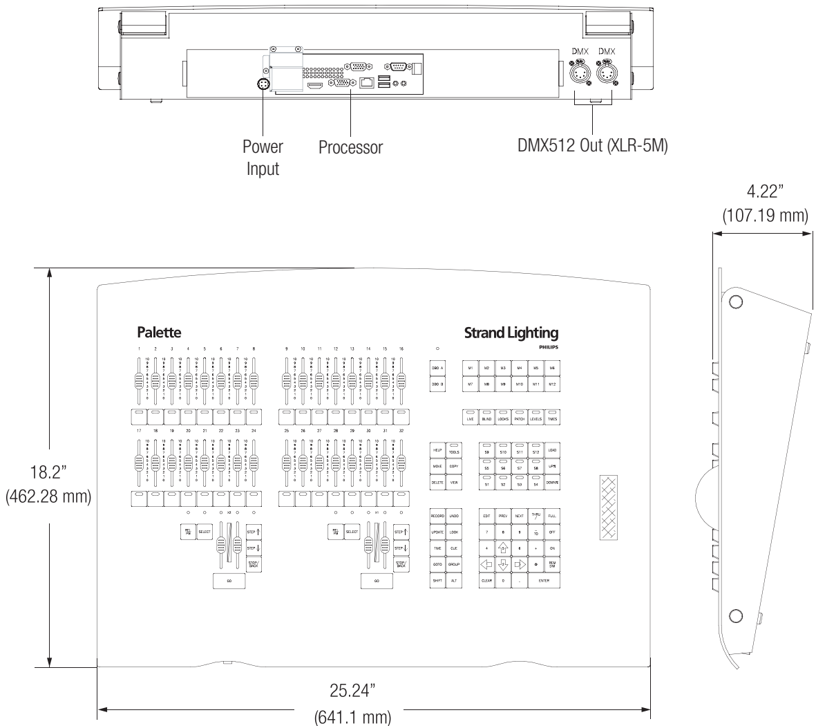
92803, 92804, 92805, 92808, 92809 classic Palette II Memory Console with 150, 250, 500, 1000 and 1500 channels with 32 submasters
